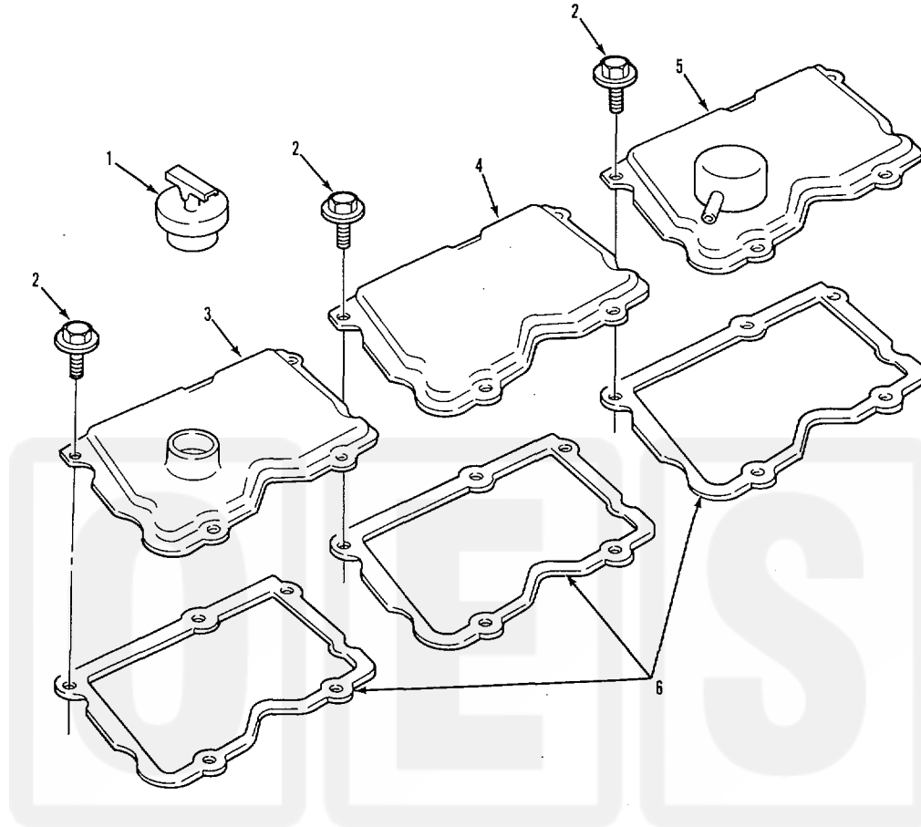
FIGURE 3. ROCKER COVERS.
